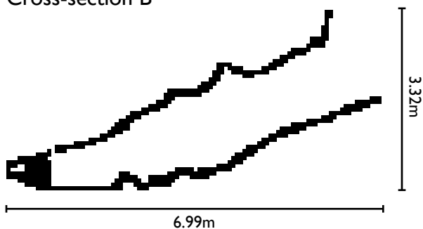
Cross-section B
