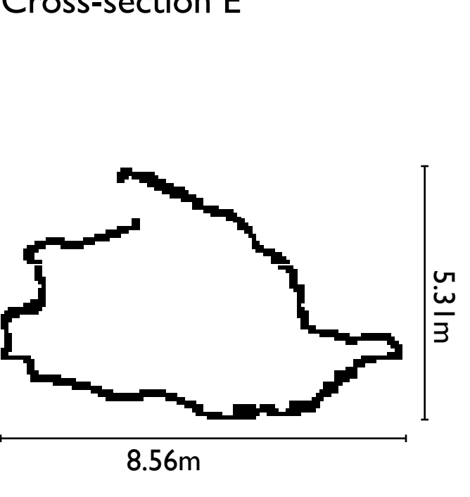
Cross-section E
