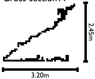
Cross-section A
